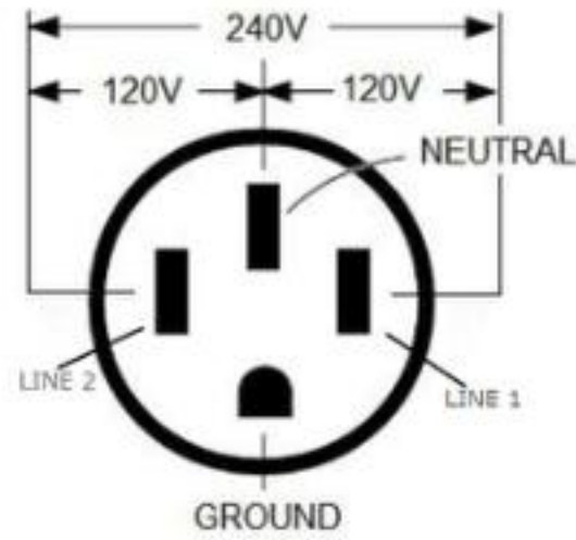
NEMA14-50R
